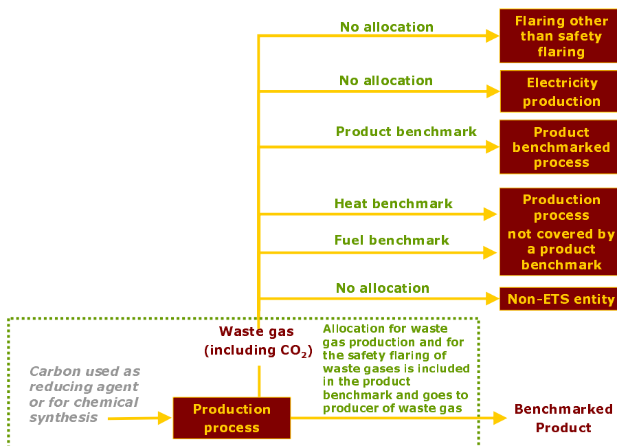
Figure 4-4 Overview of allocation in case of production of waste gases within the boundaries of a product benchmark
