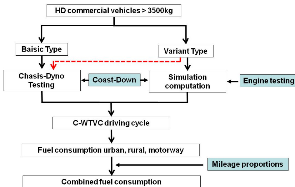
Figure 29: General overview Chinese CO 2 measurement standard (20)
