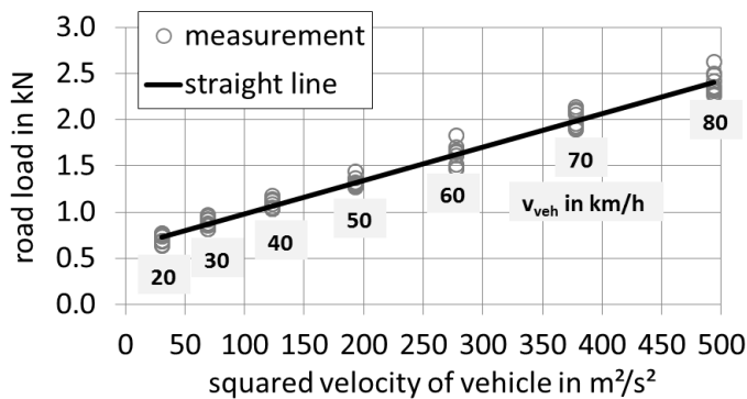
Figure 113: Road load force according to EPA-HQ-OAR-2010-0162 (no consideration of wind)
