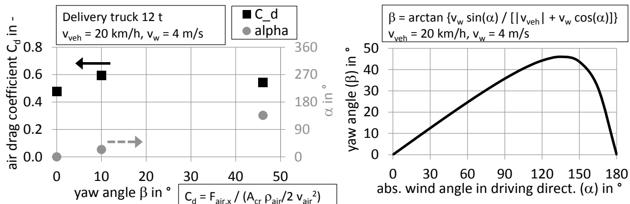
Figure 56: Air drag coefficient as function of yaw angle for a delivery truck 12 t (results from CFD simulation at TUG)
