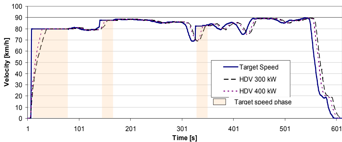
Figure 3: Motorway part of the Common Short Test cycle (CST) as an example of a target speed cycle which allows individual acceleration behaviour instead of a predefined vehicle speed trace
