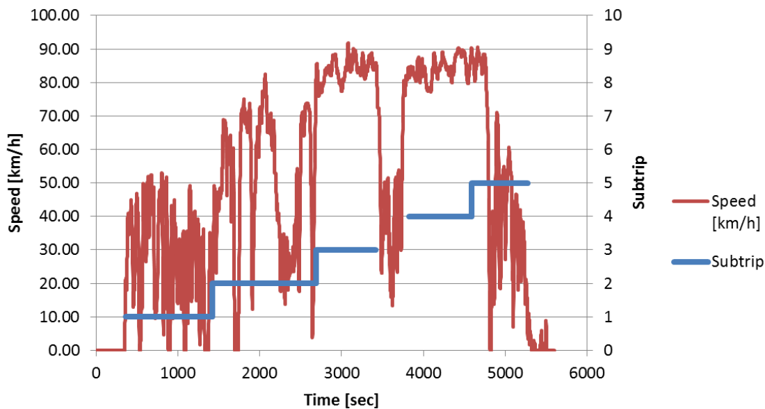
Figure 43: Speed profile and subtrip division from one of the PEMS on-road tests
