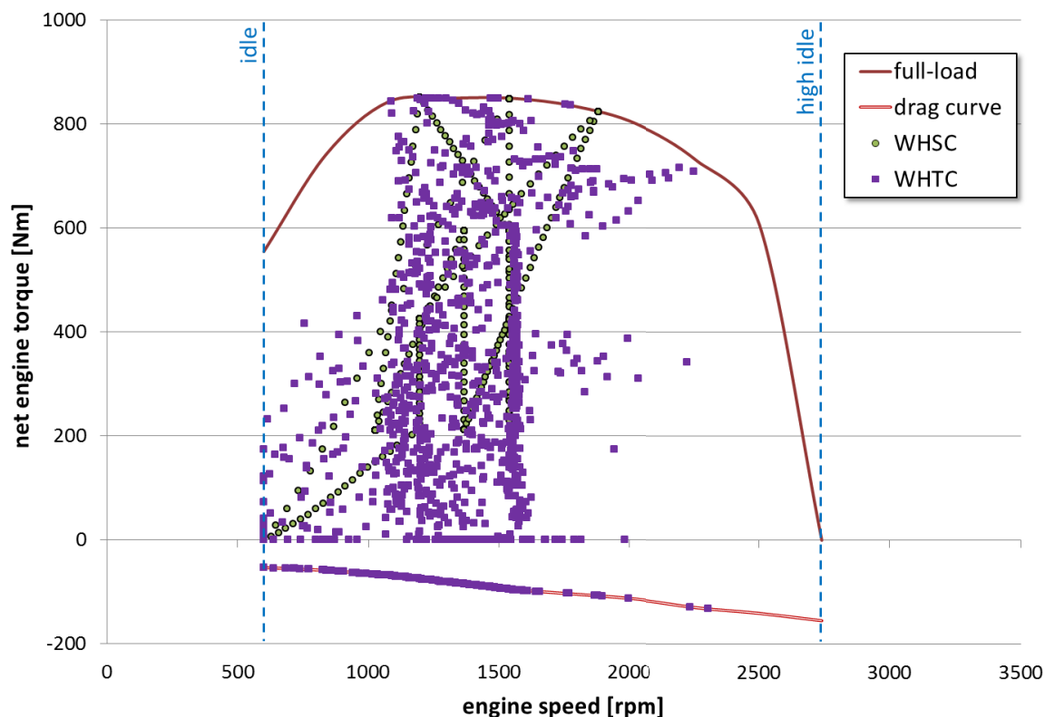
Figure 6: Example of engine operation points in the WHTC, WHSC and in the fuel map for CO 2 certification
