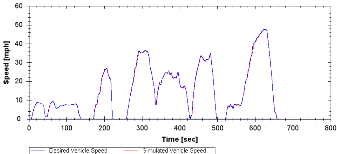
Figure 16: California Air Resource Board transient vehicle cycle
