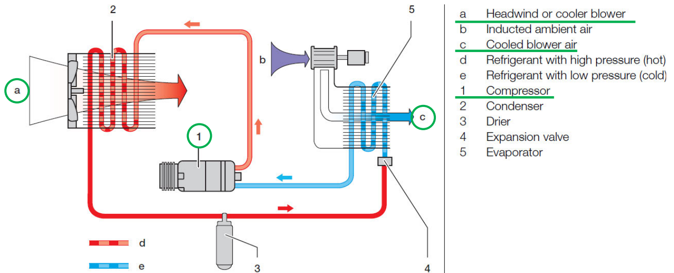
Figure 74: Scheme of an air conditioning unit (58 p. 342)
