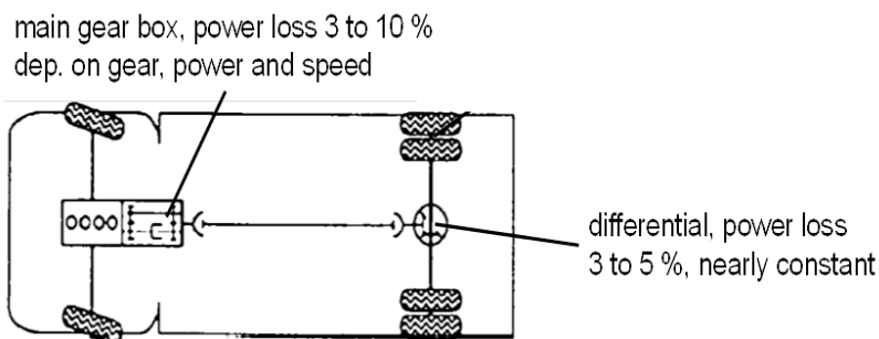
Figure 63: Typical drivetrain layout for a HDV with friction clutch and one powered axle (4x2, 6x2, 8x2) (54 p. 437)
