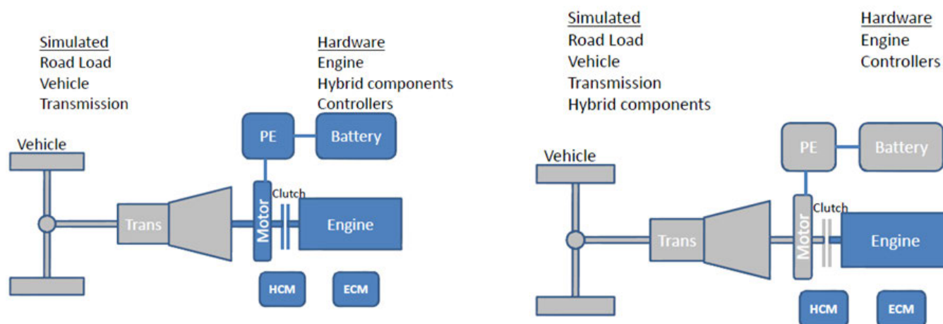
Figure 11: Schematic picture of a power pack test (left) and a HILS test (right), where the components marked in blue are applied on an engine test bed to run speed and torque cycles, (12)
