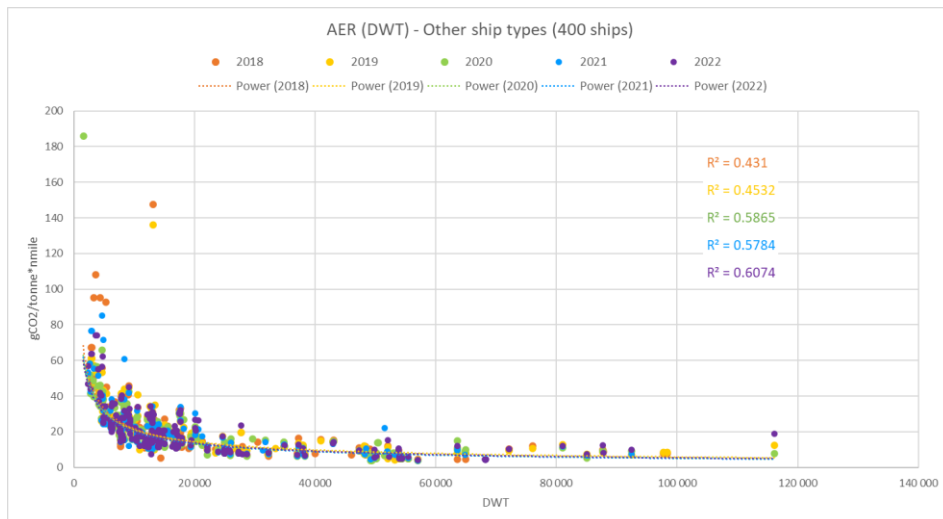
Figure 52: Plot of attained AER values of other ship types over the five reporting years and associated trendlines
