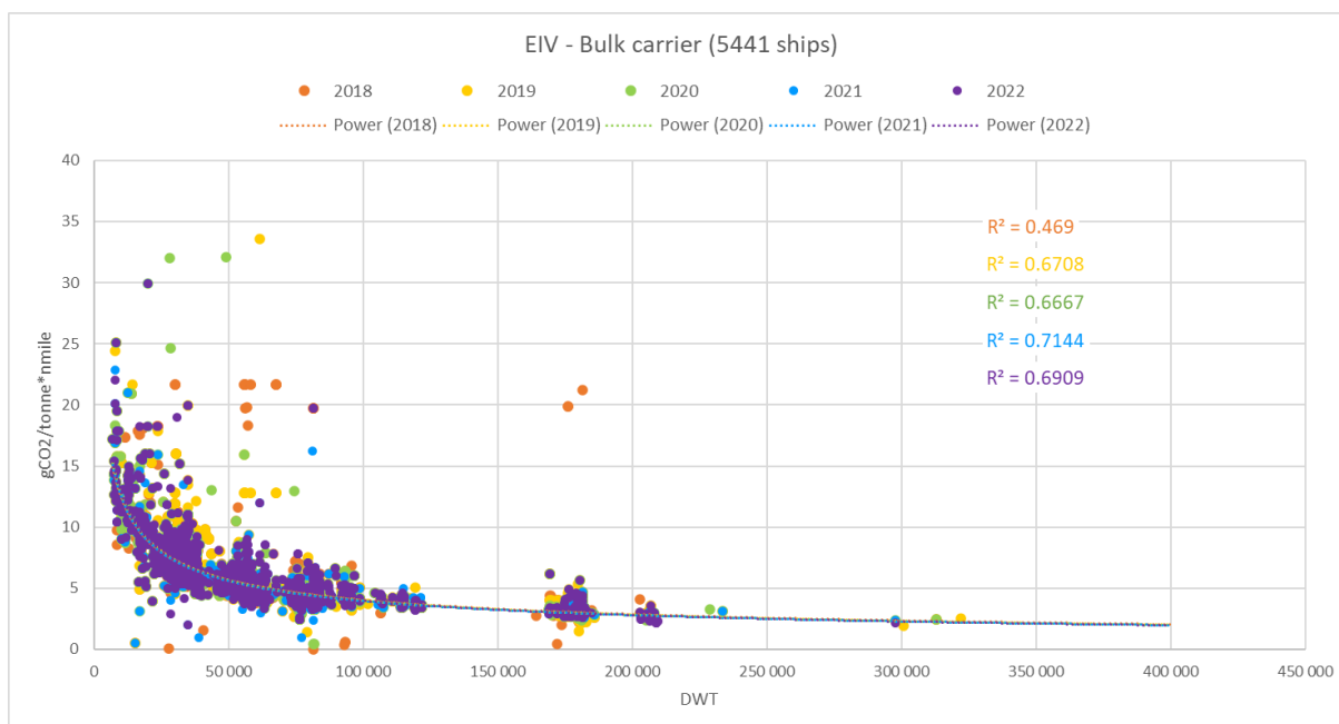
Figure 21: Plot of attained EIV values for bulk carriers over the five reporting years and associated trendlines
